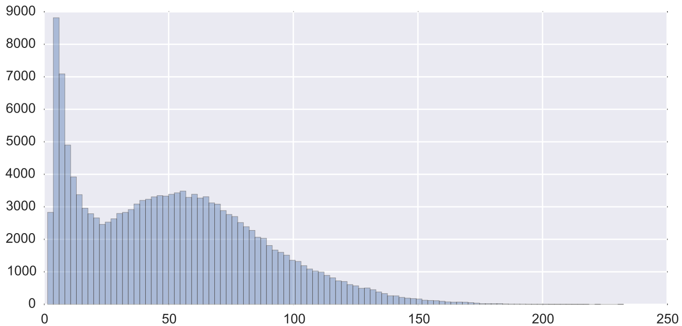
Subject 25719 tSNR inside the mask
