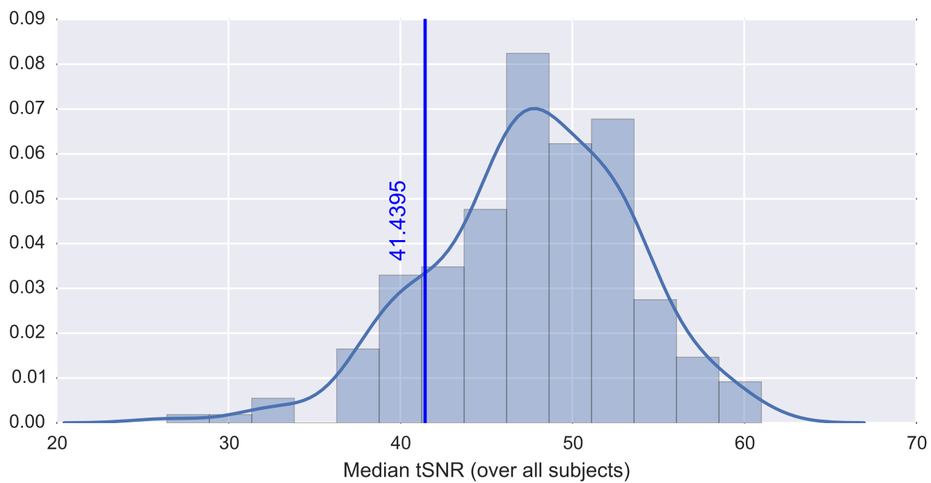
Subject 25194 tSNR inside the mask
