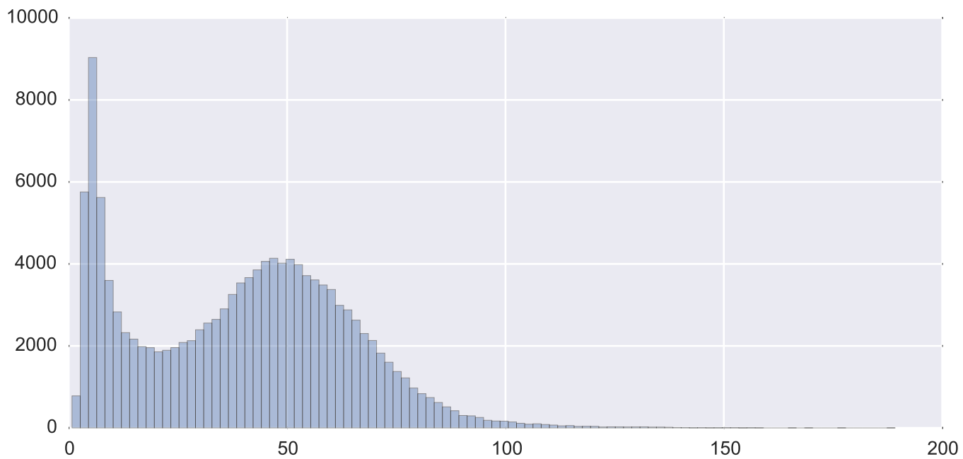
Subject 25194 tSNR inside the mask
