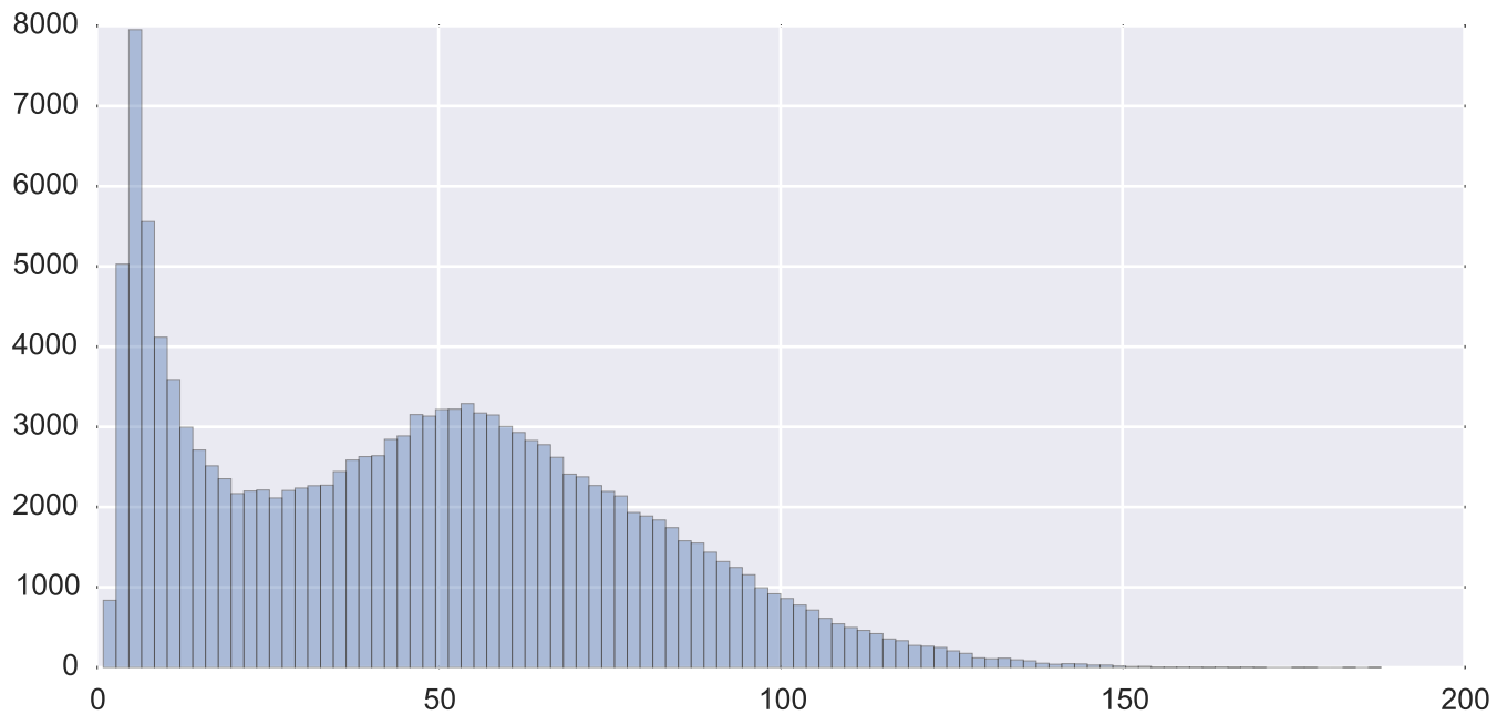
Subject 23963 tSNR inside the mask
