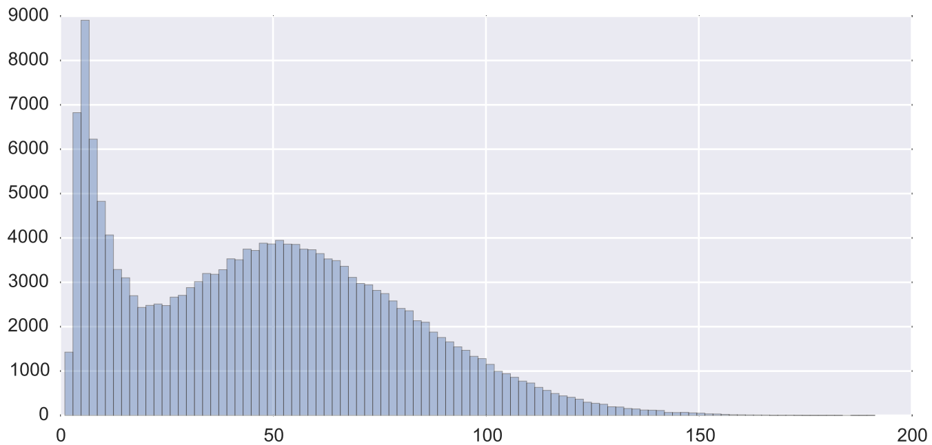
Subject 23629 tSNR inside the mask
