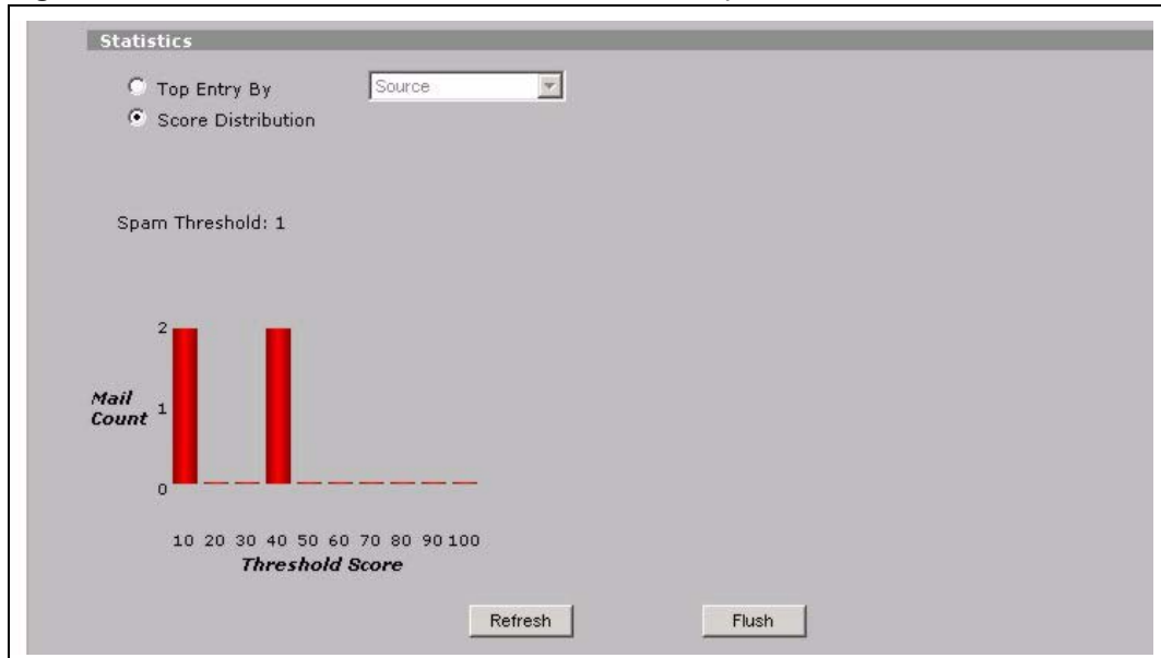
Figure 285 REPORTS > THREAT REPORTS > Anti-Spam > Score Distribution
