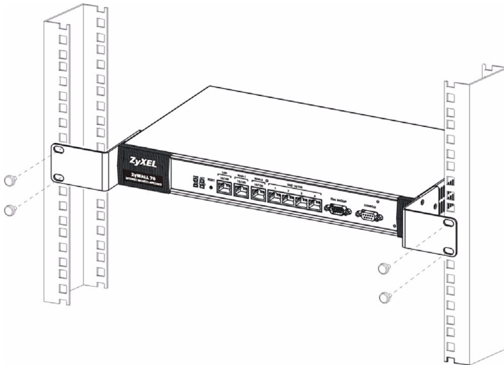
Figure 452 Rack Mounting
