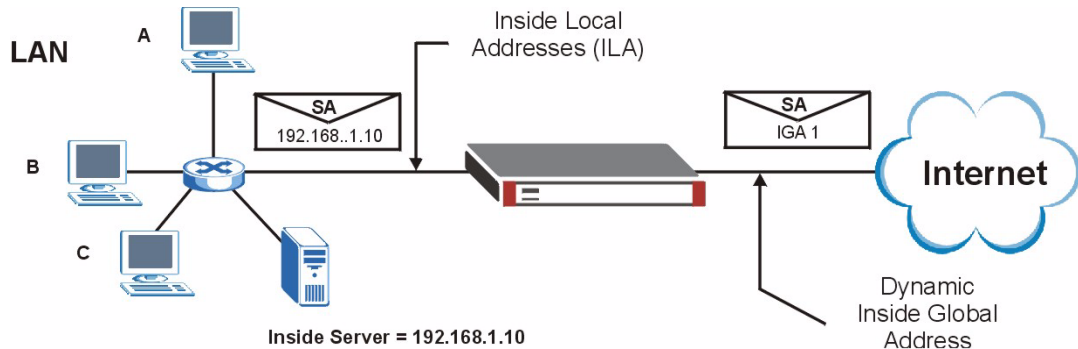
Figure 372 NAT Example 2
