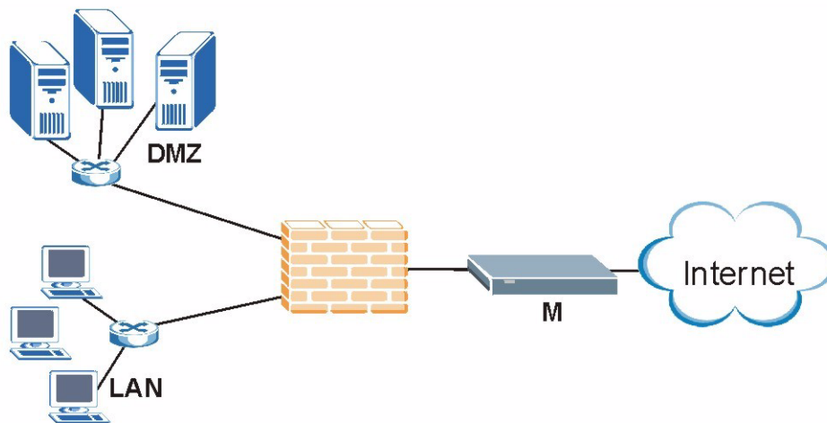
Figure 134 Network Intrusions
