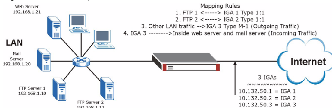
Figure 374 NAT Example 3
