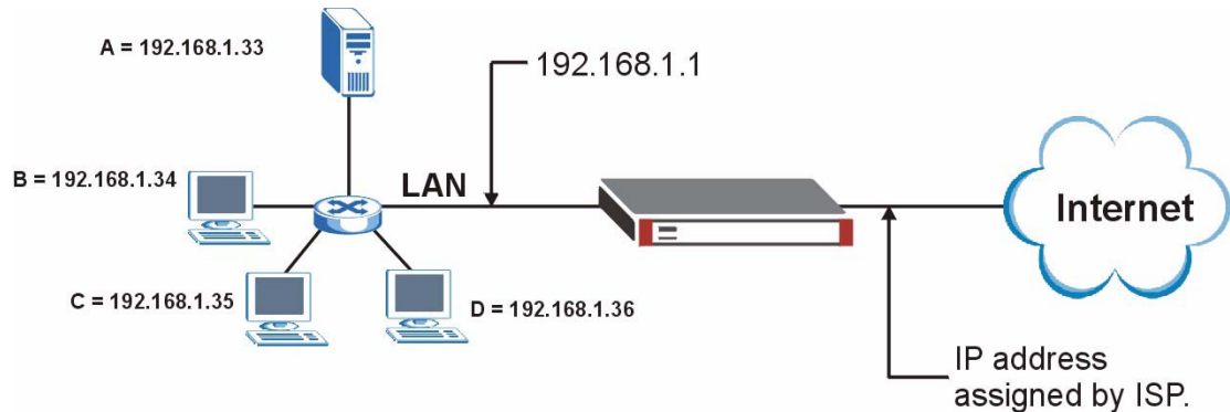
Figure 220 Multiple Servers Behind NAT Example
