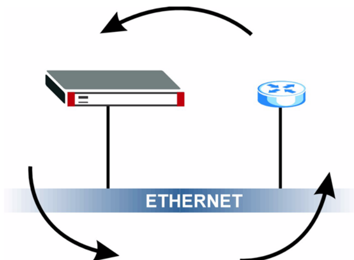
Figure 62 Bridge Loop: Bridge Connected to Wired LAN
