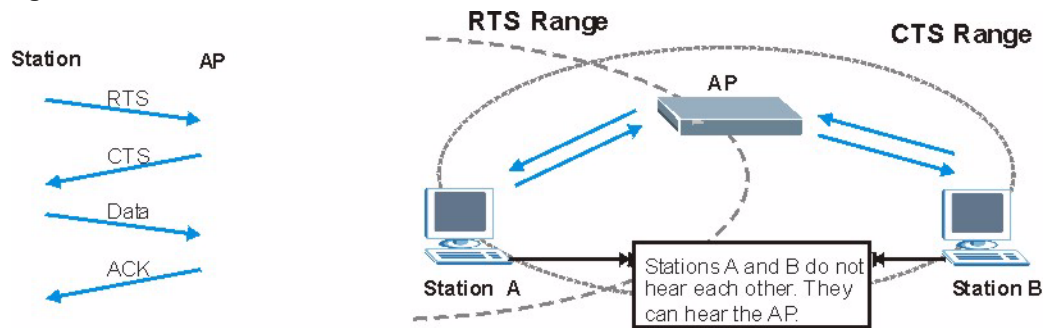
Figure 487 RTS/CTS
