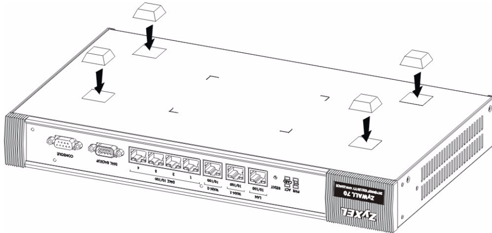
Figure 450 Attaching Rubber Feet
