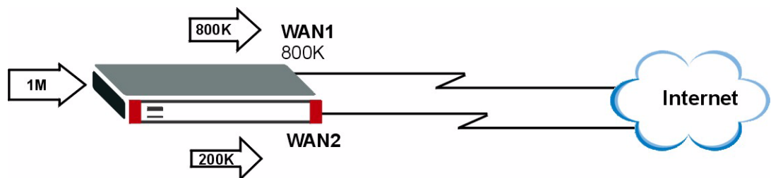
Figure 68 Spillover Algorithm Example
