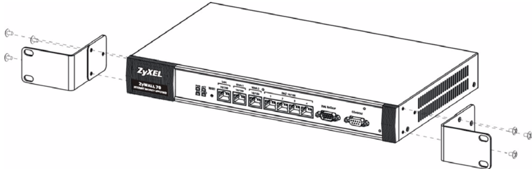
Figure 451 Attaching Mounting Brackets and Screws
