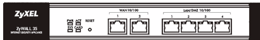
Figure 5 ZyWALL 35 Front Panel
