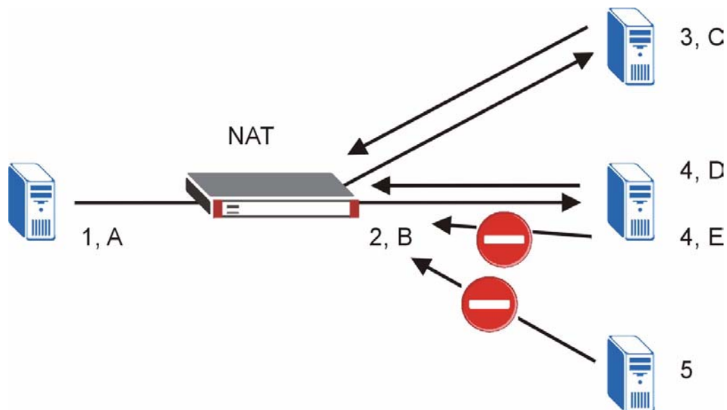
Figure 216 Port Restricted Cone NAT Example
