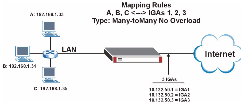
Figure 379 NAT Example 4
