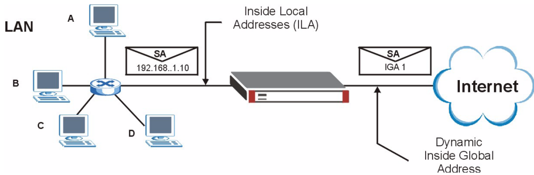
Figure 370 NAT Example 1
