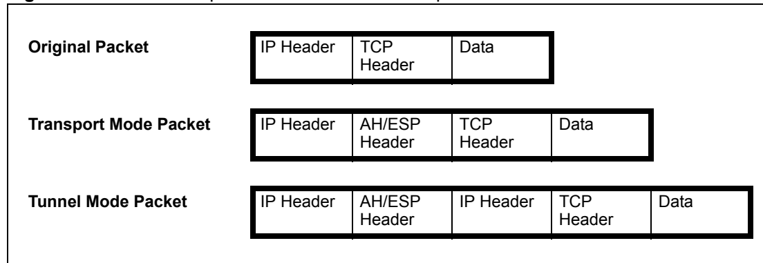
Figure 183 VPN: Transport and Tunnel Mode Encapsulation
