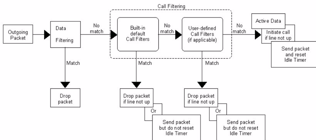
Figure 385 Outgoing Packet Filtering Process
