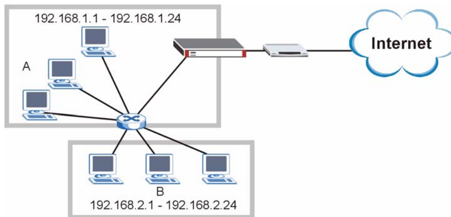
Figure 230 Subnet-based Bandwidth Management Example
