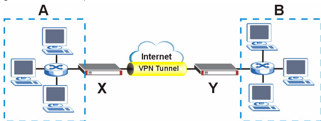
Figure 172 VPN: Example
