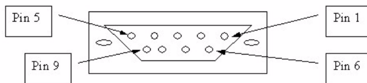
Figure 449 Console/Dial Backup Port Pin Layout
