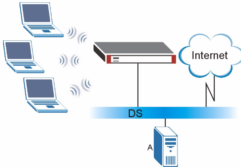
Figure 97 WPA with RADIUS Application Example
