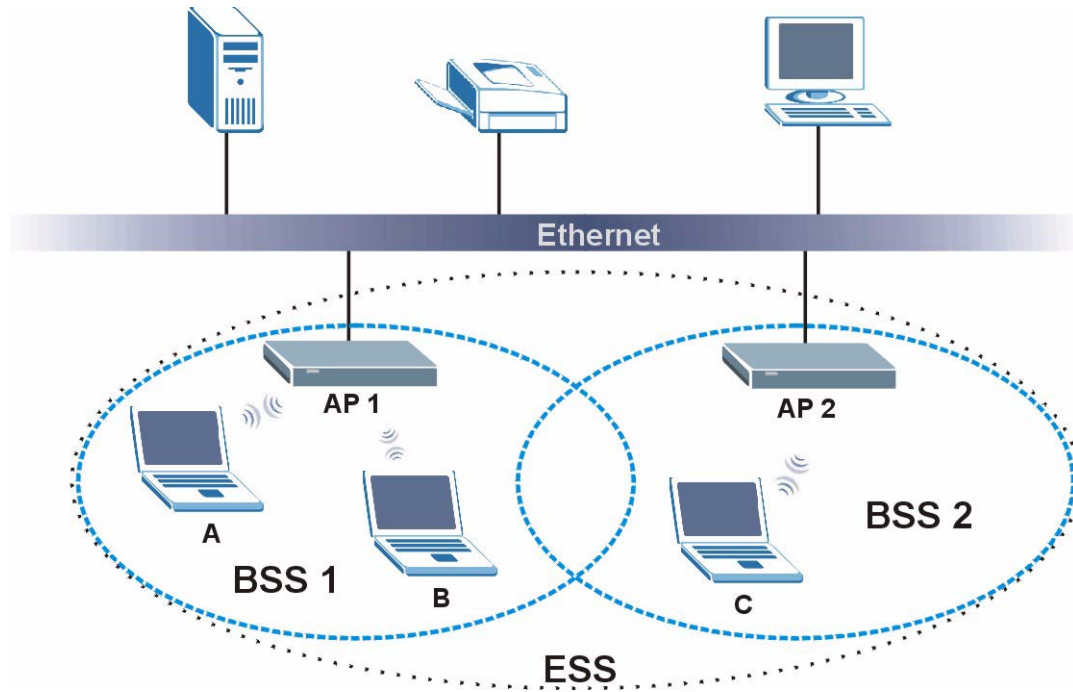
Figure 486 Infrastructure WLAN
