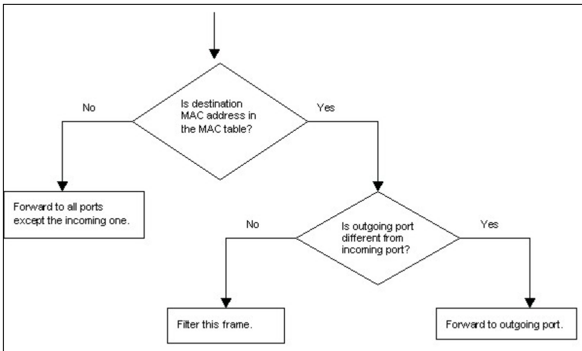
Figure 23-1 MAC Table Flowchart
