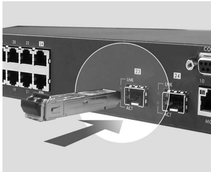
Figure 3-2 Transceiver Installation Example
