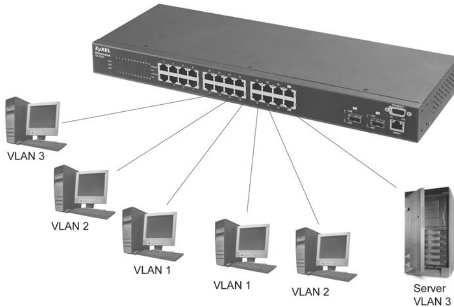
Figure 1-5 Shared Server Using VLAN Example
