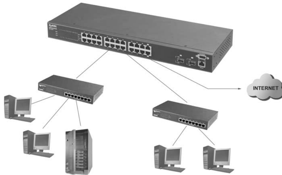
Figure 1-2 Bridging Application
