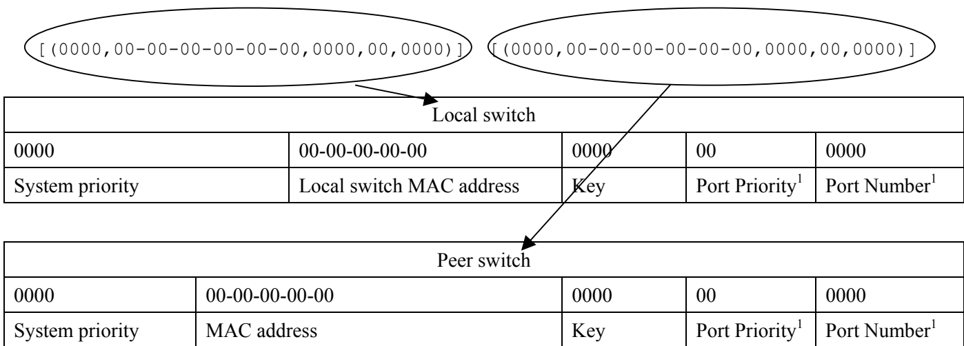
Figure 13-1 Aggregation ID
