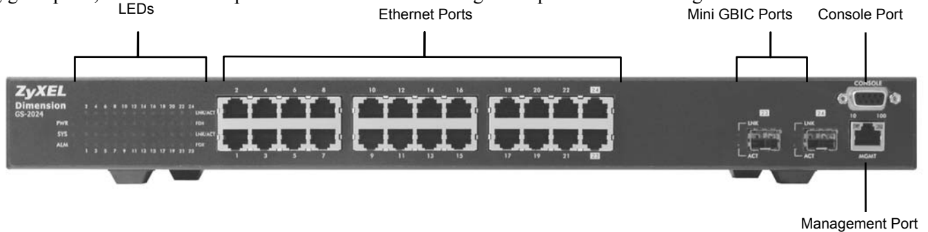
Figure 3-1 GS-2024 Front Panel
