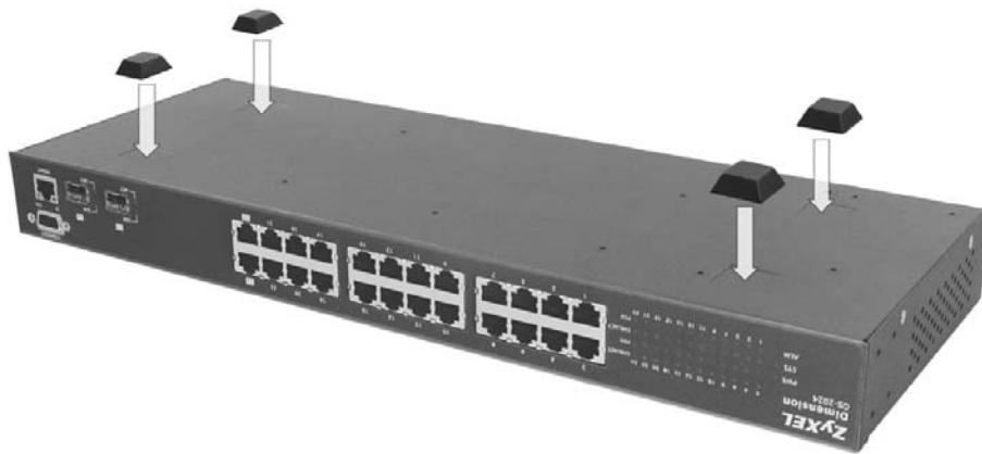
Figure 2-1 Attaching Rubber Feet
