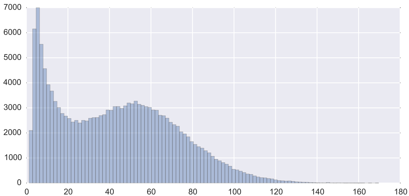
Subject 27880 tSNR inside the mask
