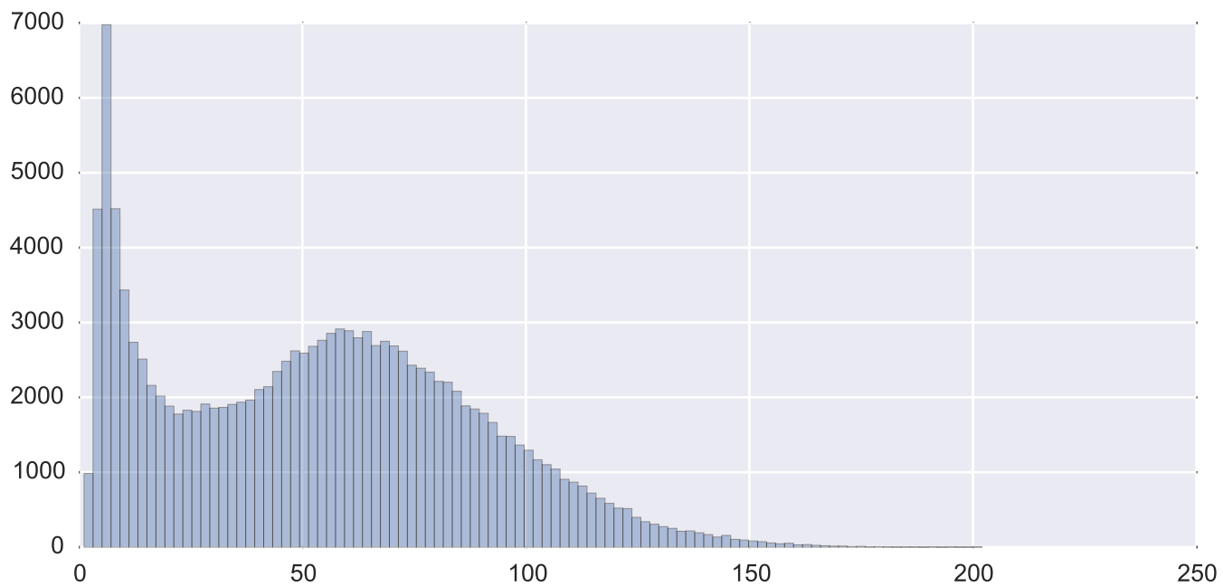
Subject 24844 tSNR inside the mask
