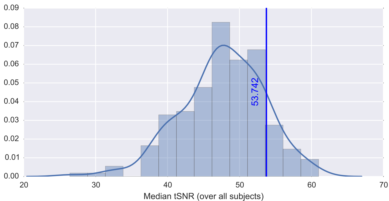
Subject 24844 tSNR inside the mask
