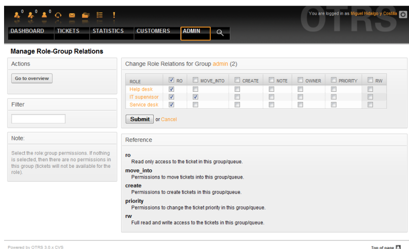
Figure 5.14. Change Role relations for a Group.
