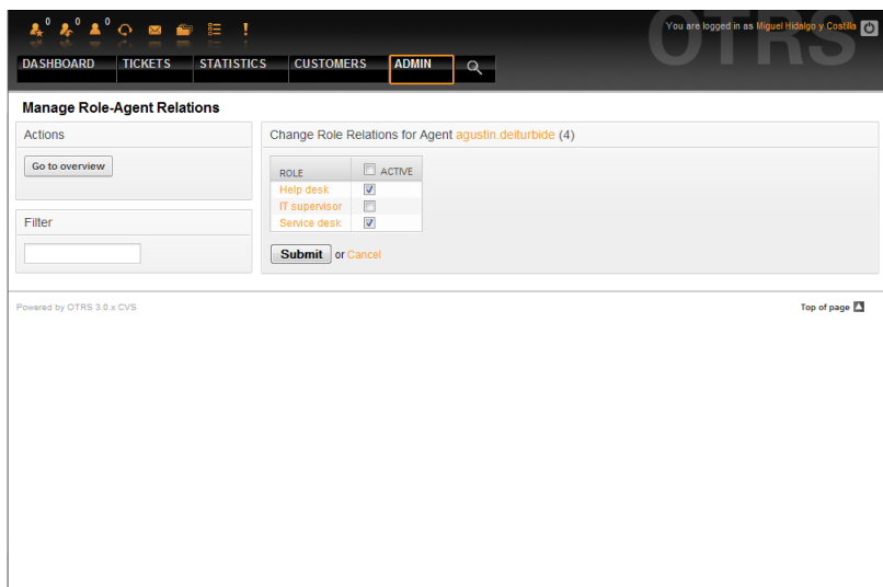
Figure 5.10. Change the Roles associated with an Agent.
