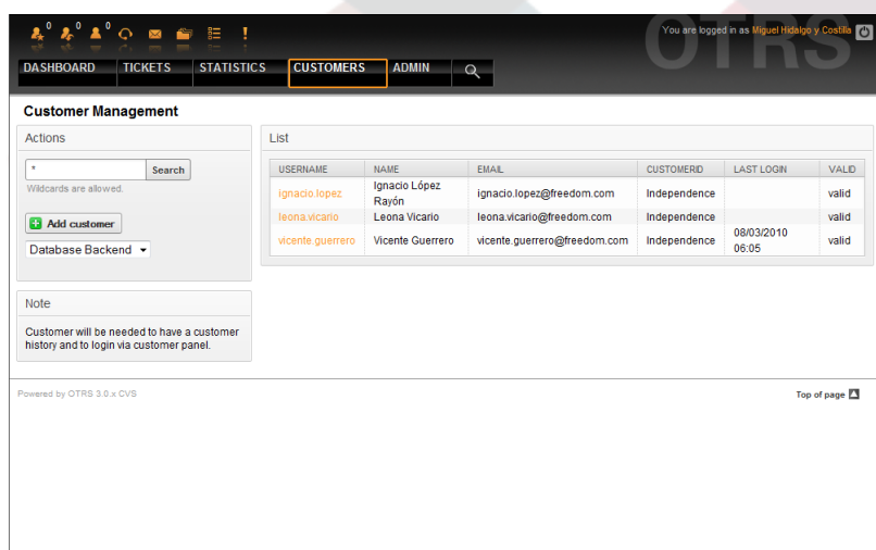
Figure 5.14. Customer management.
