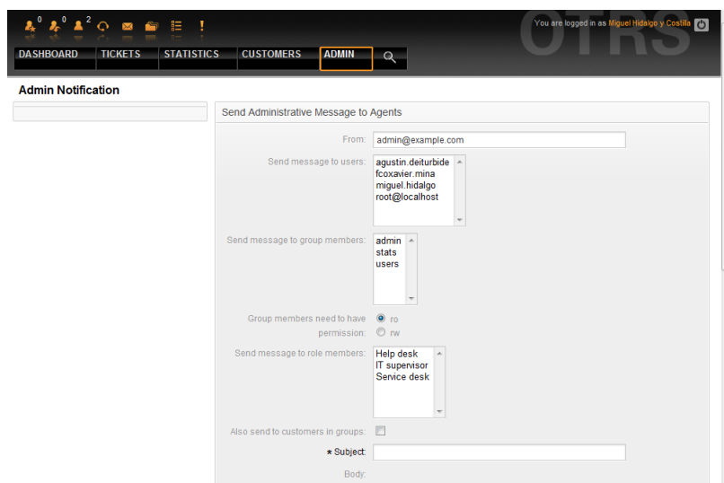
Figure 5.53. Admin notification.
