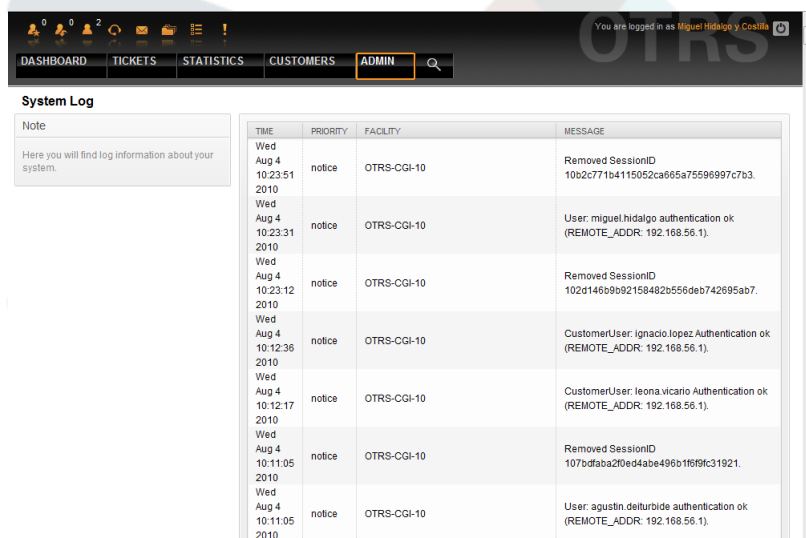
Figure 5.56. System Log.
