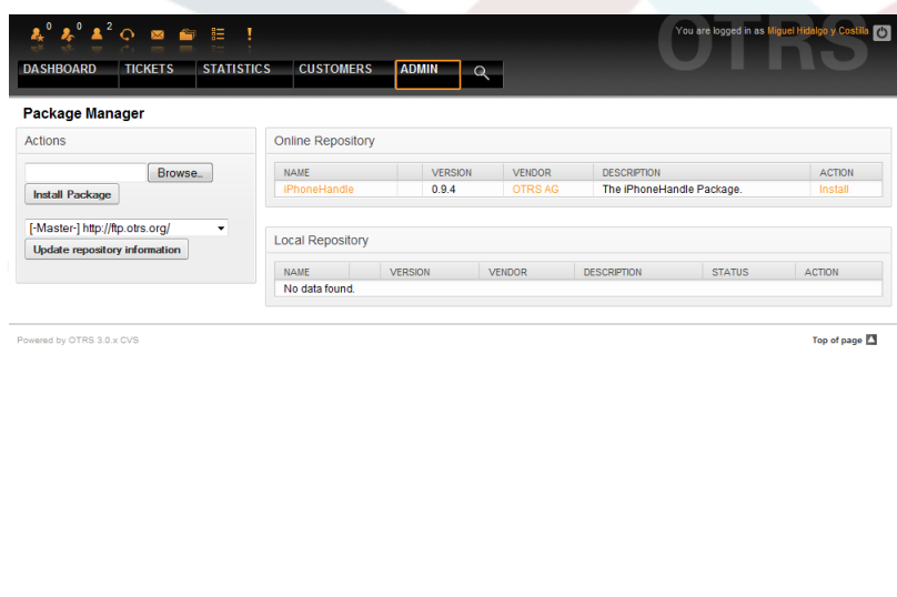
Figure 5.58. Package Manager.
