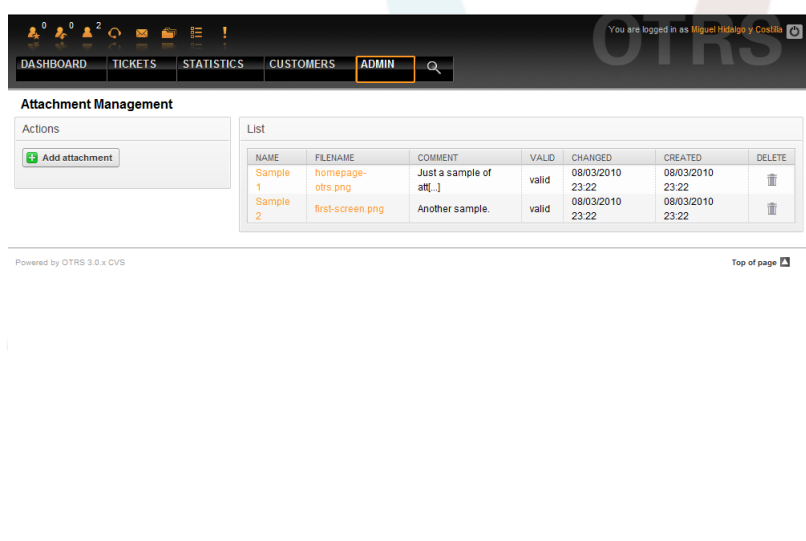
Figure 5.24. Attachments management.
