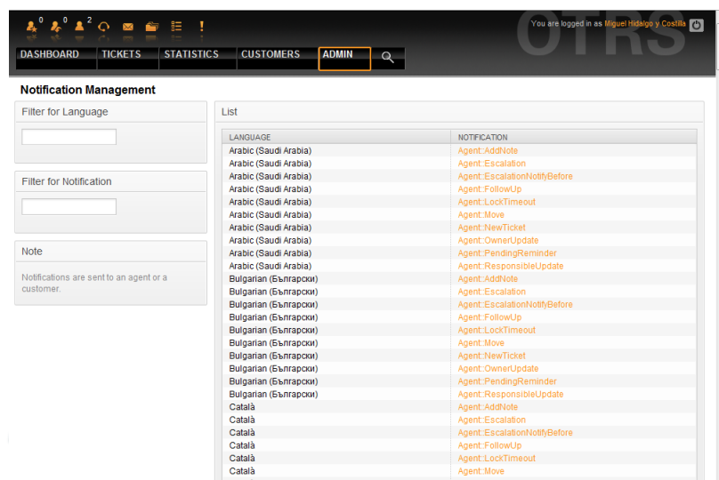
Figure 5.40. Notification management.
