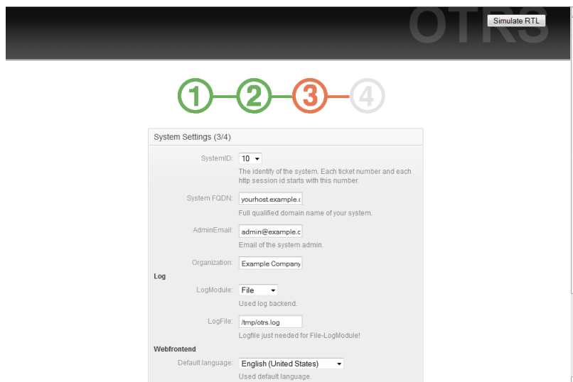
Figure 3.7. System settings.
