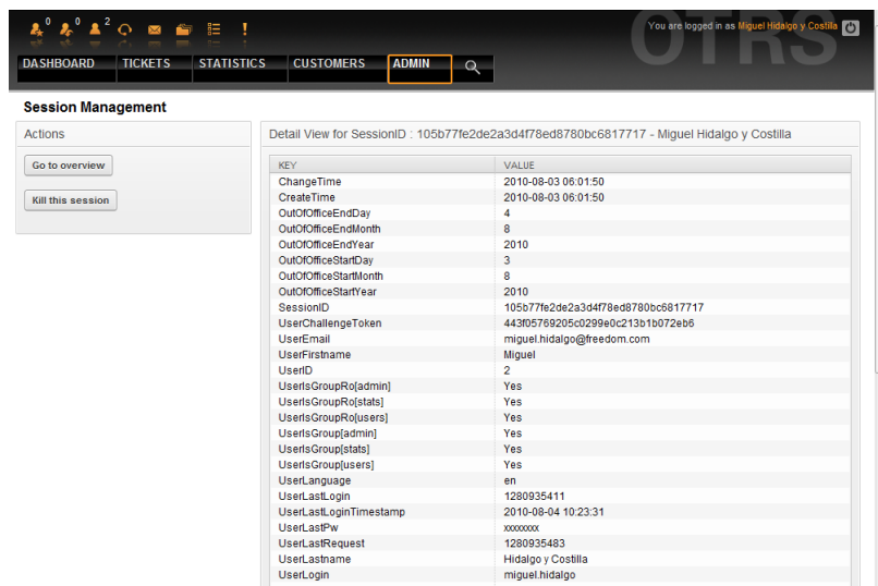
Figure 5.55. Session details.
