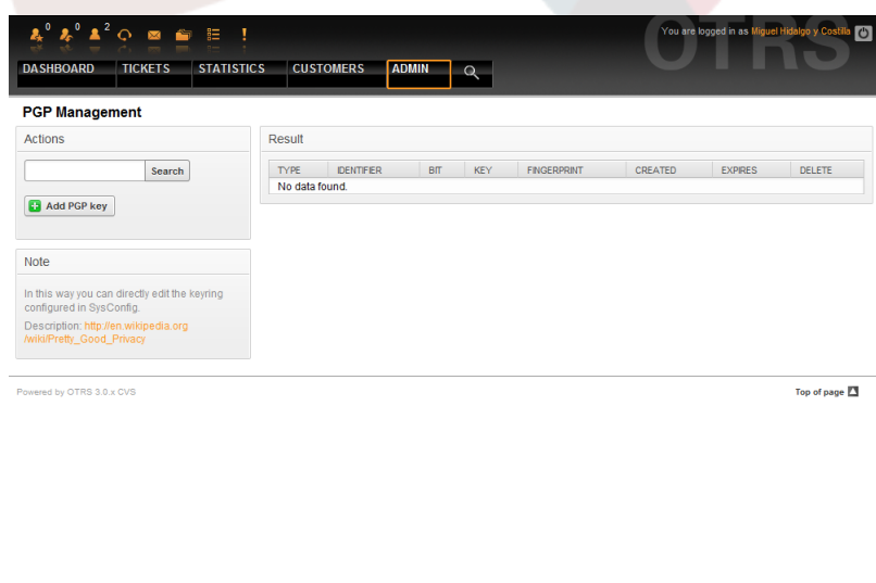
Figure 5.45. PGP management.
