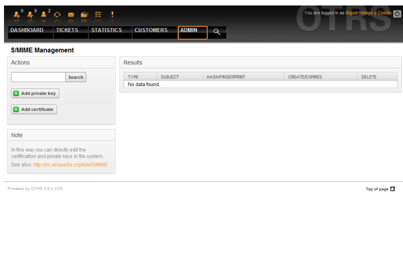
Figure 5.44. S/MIME management.
