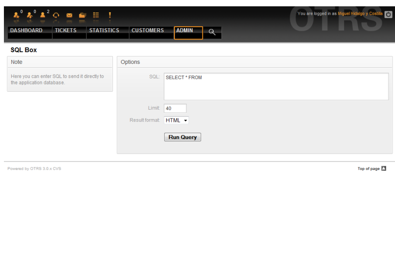
Figure 5.57. SQL Box.
