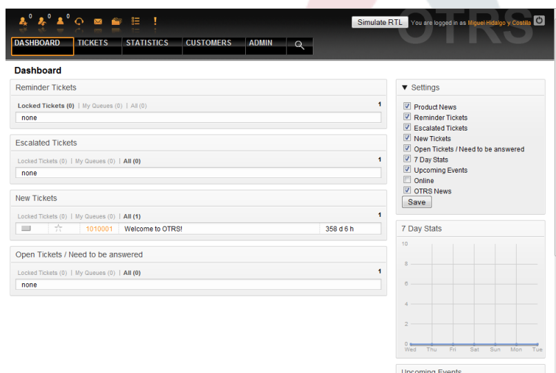
Figure 4.6. Dashboard Settings.
