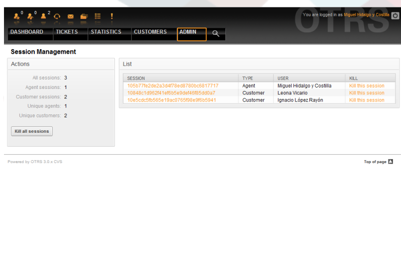
Figure 5.54. Session management.
